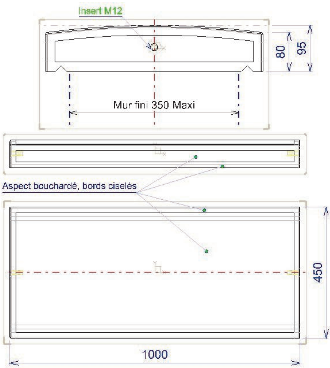
100 x 45 x 8 / 9.5 cm ; 90 kg.
